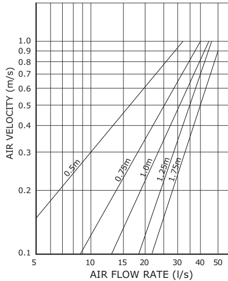
VERTICAL DIFFUSION AT 6°C COOLING
