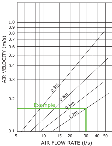
VERTICAL DIFFUSION AT 3°C COOLING
