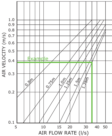
VERTICAL DIFFUSION AT 3°C COOLING
