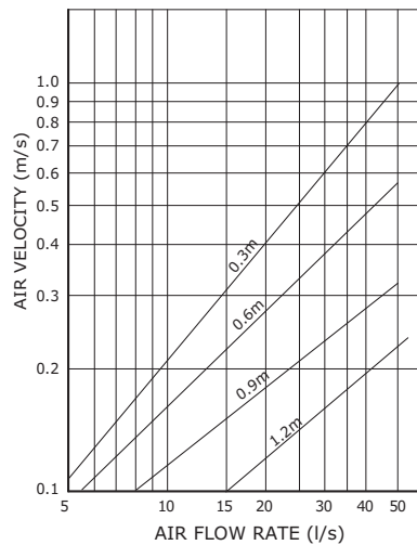
VERTICAL DIFFUSION AT 6°C COOLING
